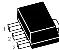
1.Base 2.Collector 3.Emmitter SOT-89 Plastic Package
