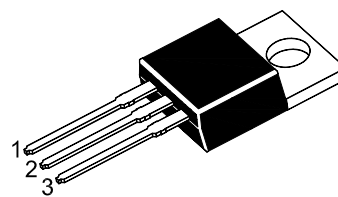
1.Input 2.Common 3.Output TO-220 Plastic Package
