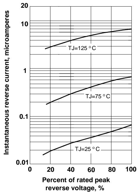
Typical reverse characteristics
